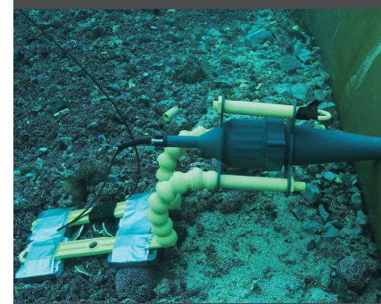
PLMEOD™ being used to detonate a US MK 25 Ground Mine. (Courtesy of the Royal Norwegian Navy).
