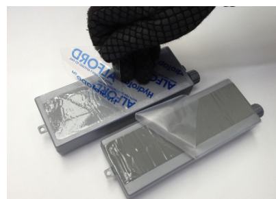
HydroTape™ (left), Breacher's Tape™ (right) applied to a charge
